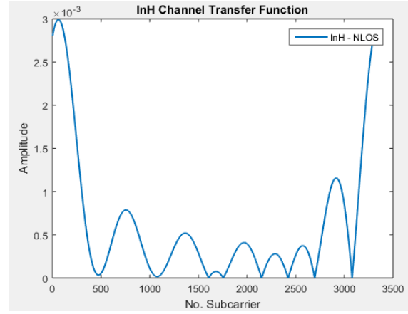
Fig. 5. The transfer function of InH scenario
