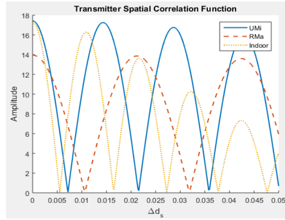
Fig. 6. The correlation properties in BS side
