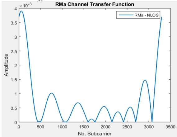
Fig. 4. The transfer function of RMa
