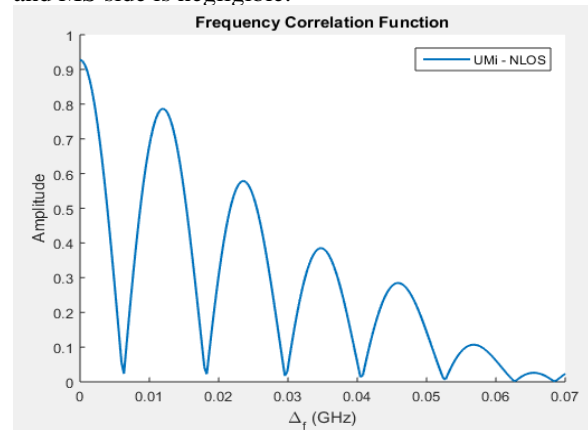
Fig. 9. The frequency ACF of UMi
