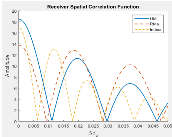
Fig. 7. The correlation properties in MS side
