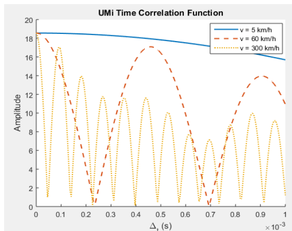
Fig. 8. The temporal ACF of UMi
