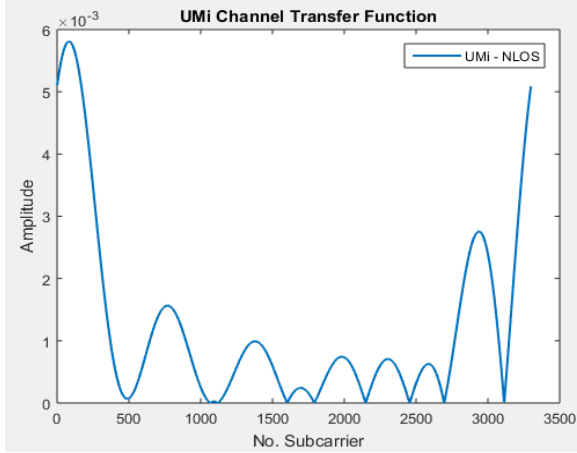
Fig. 3. The transfer function of UMi
